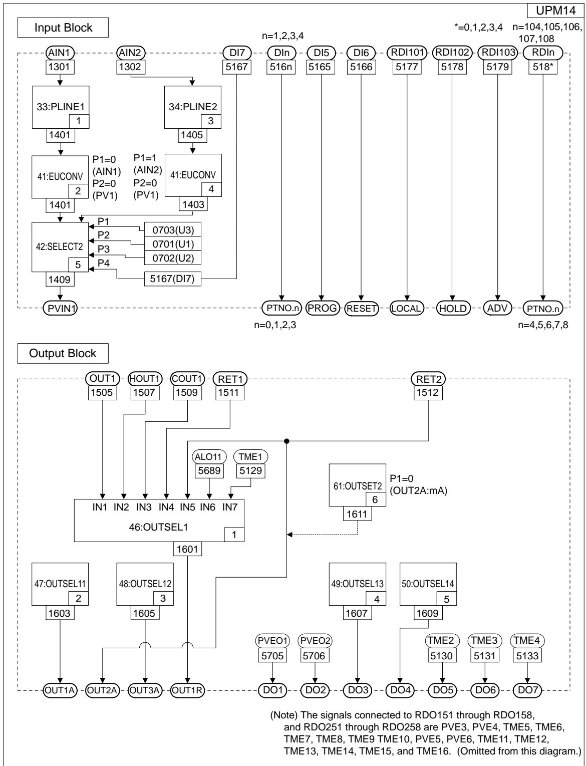
Figure 2.12 Input and Output Blocks for Loop Control with PV Switching and Two Universal Inputs (UP Mode 14)
