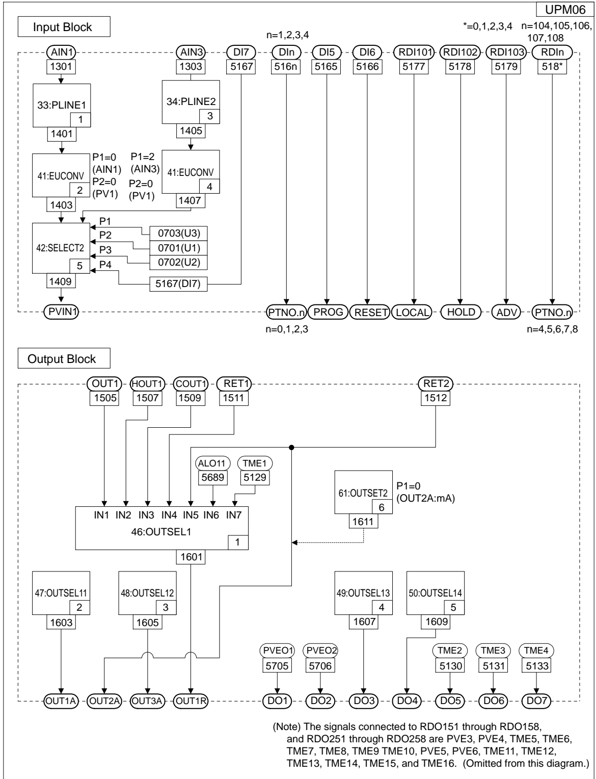
Figure 2.7 Input and Output Blocks for Loop Control with PV Switching (UP Mode 6)
