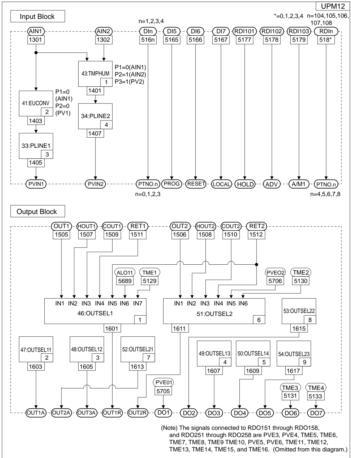
Figure 2.10 Input and Output Blocks for Temperature and Humidity Control (UP Mode 12)
