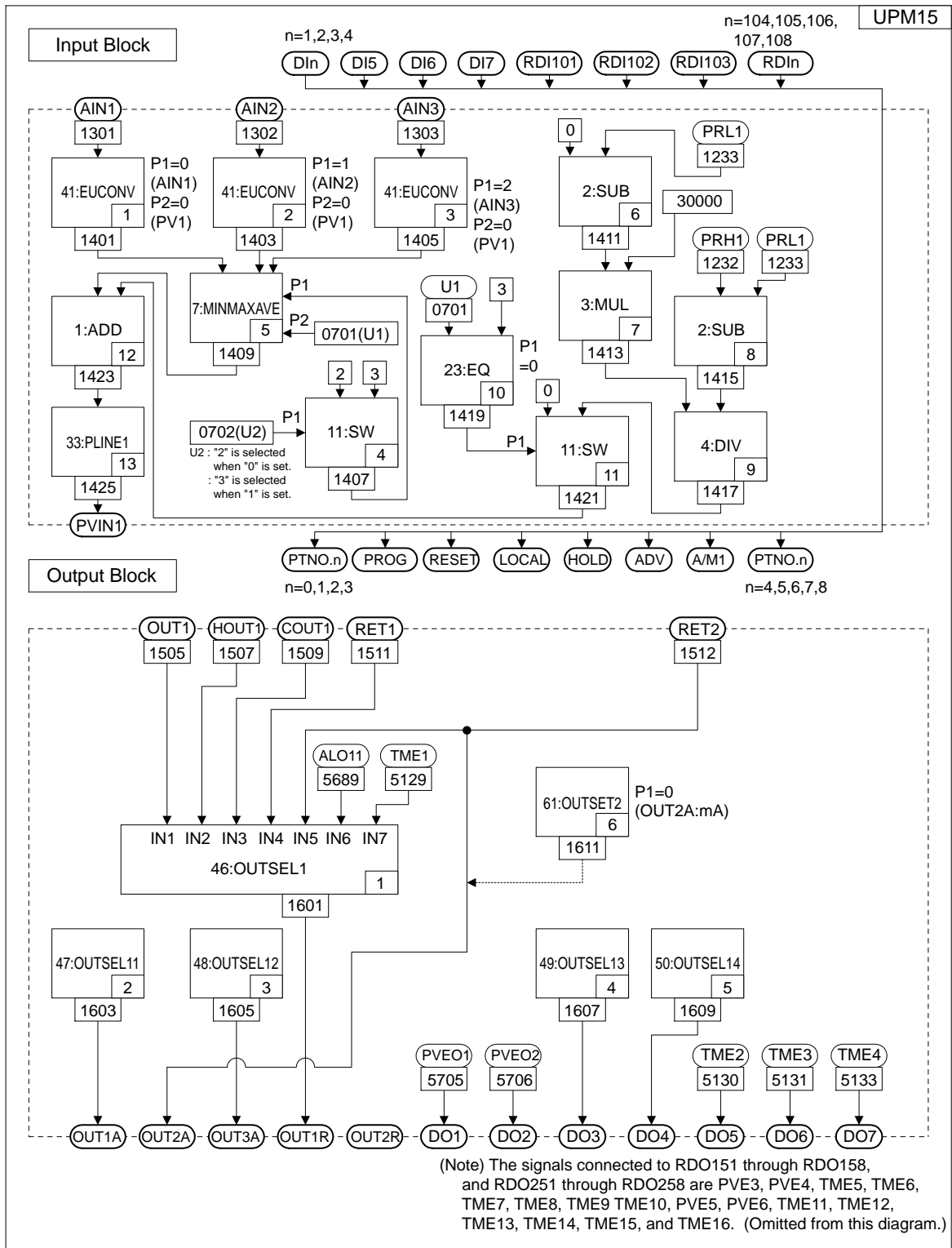
Figure 2.13 Input and Output Blocks for Loop Control with PV Auto-selector and Two Universal Inputs (UP Mode 15)
