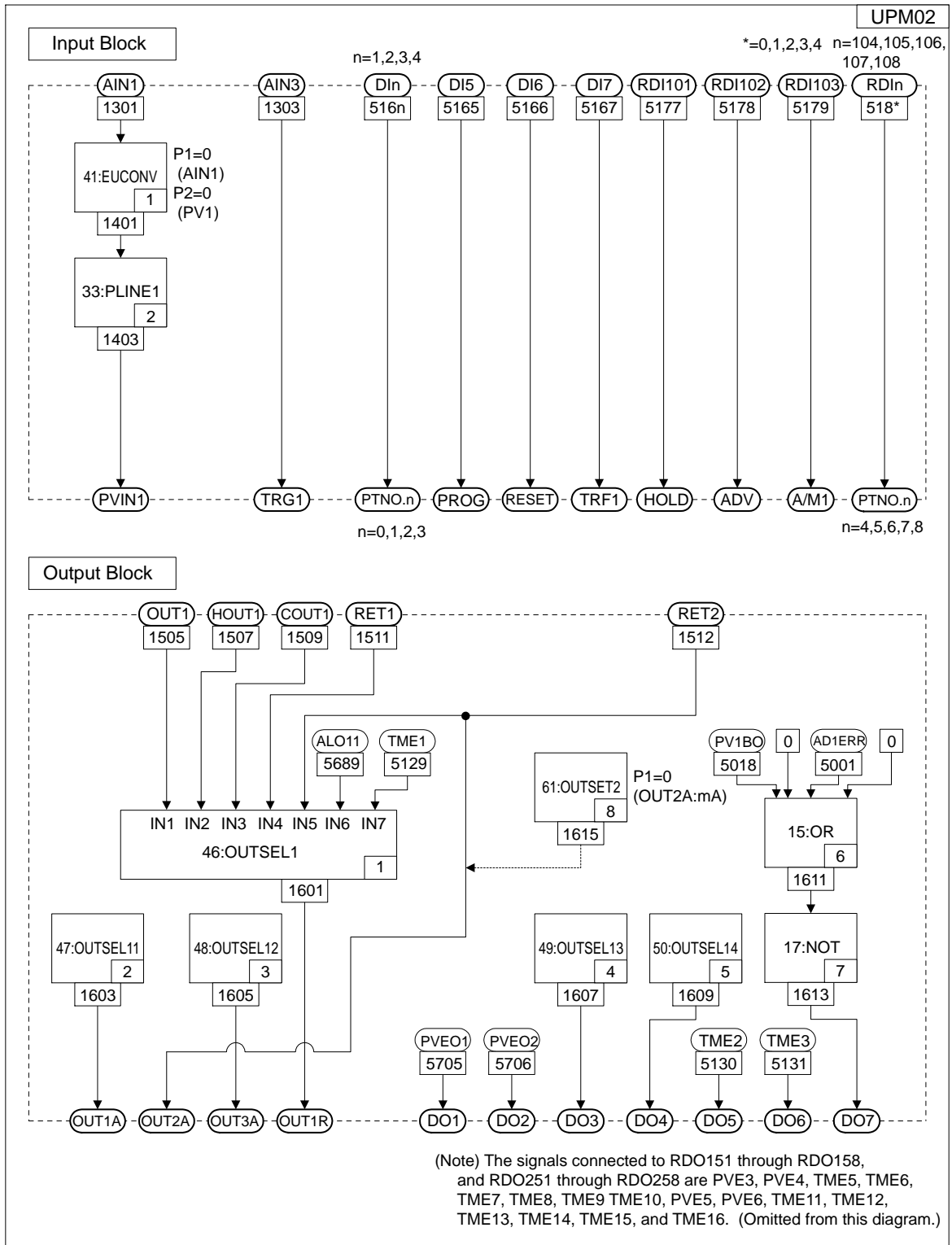
Figure 2.5 Input and Output Blocks for Cascade Primary-loop Control (UP Mode 2)
