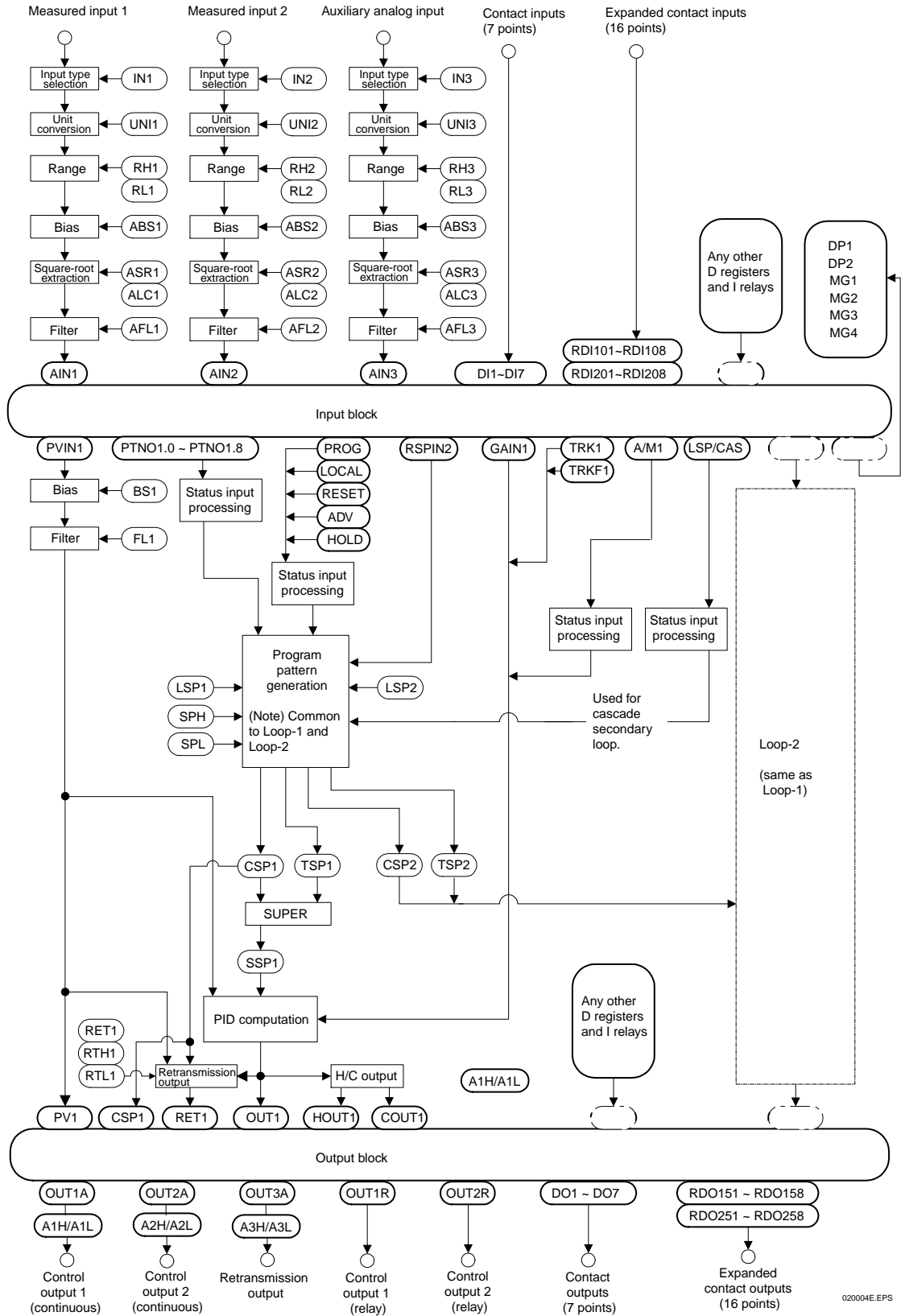
Figure 2.3 Function Block Diagram of UP750 (Whole View)
