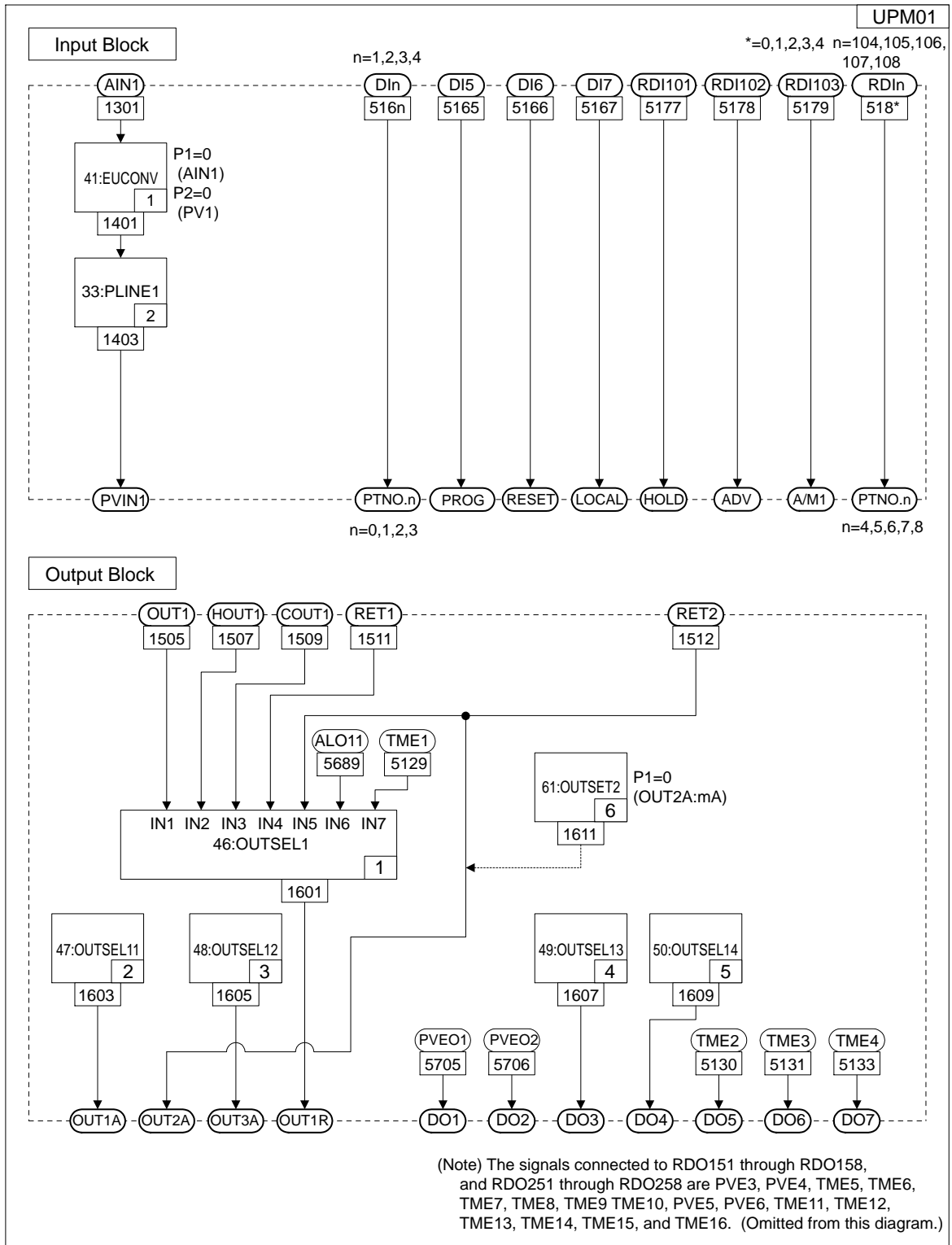
Figure 2.4 Input and Output Blocks for Single-loop Control (UP Mode 1)
