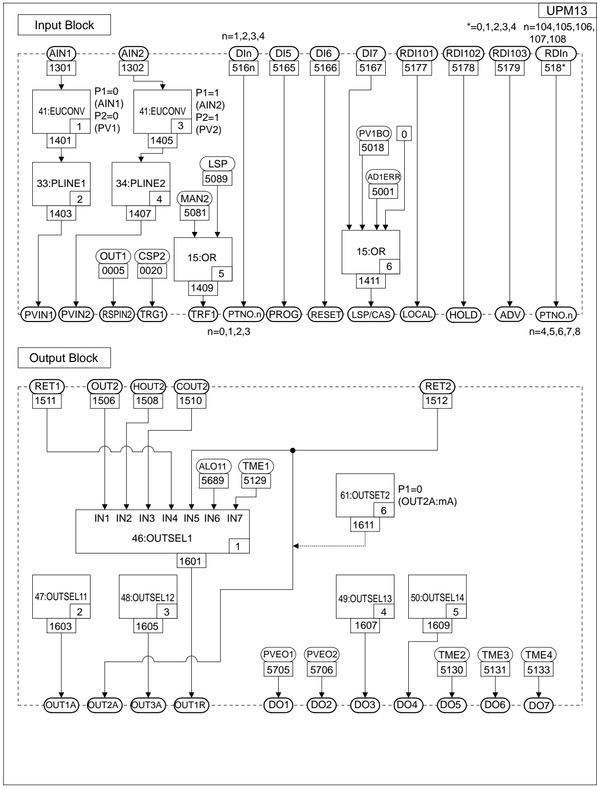
Figure 2.11 Input and Output Blocks for Cascade Control with Two Universal Inputs (UP Mode 13)
