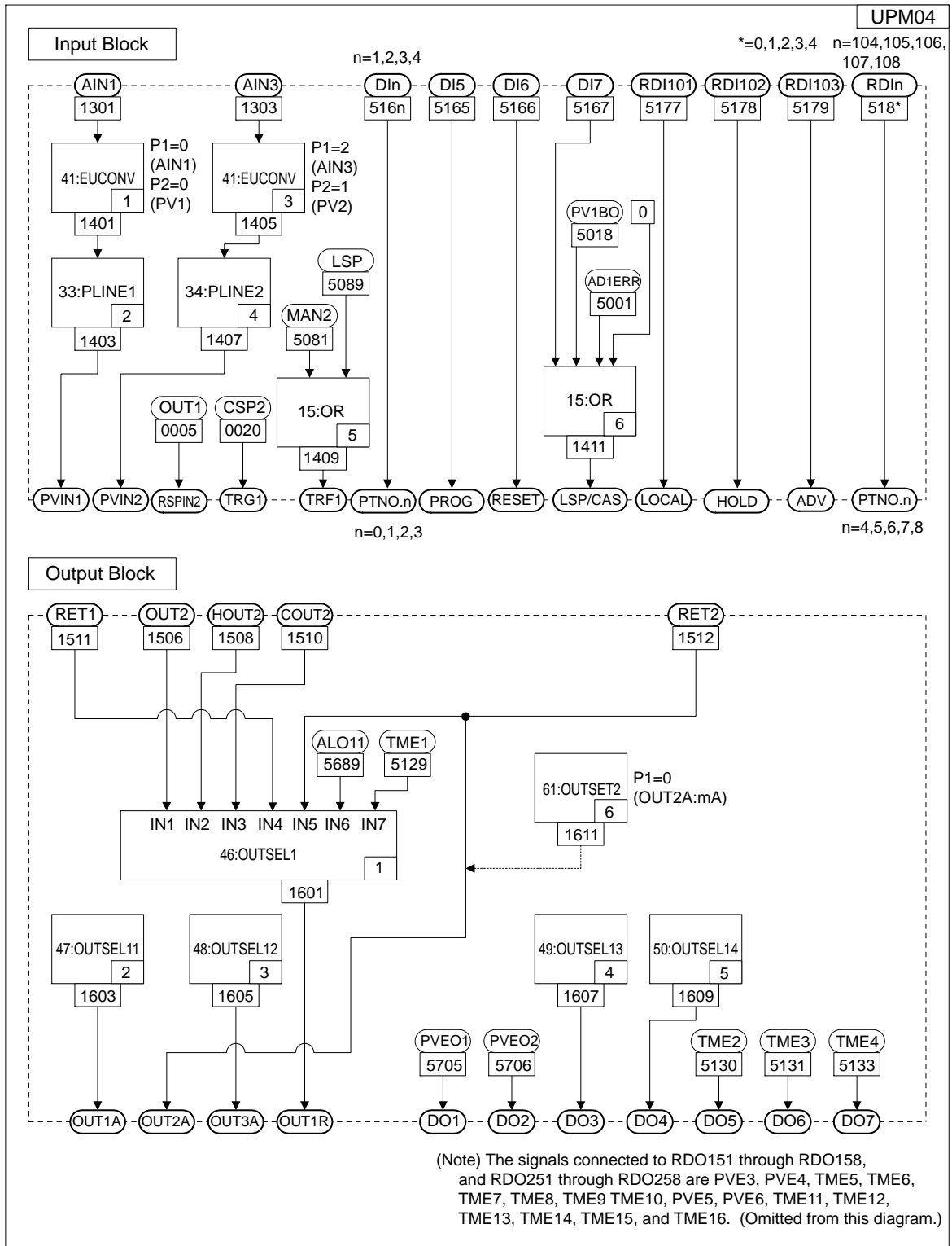
Figure 2.6 Input and Output Blocks for Cascade Control (UP Mode 4)
