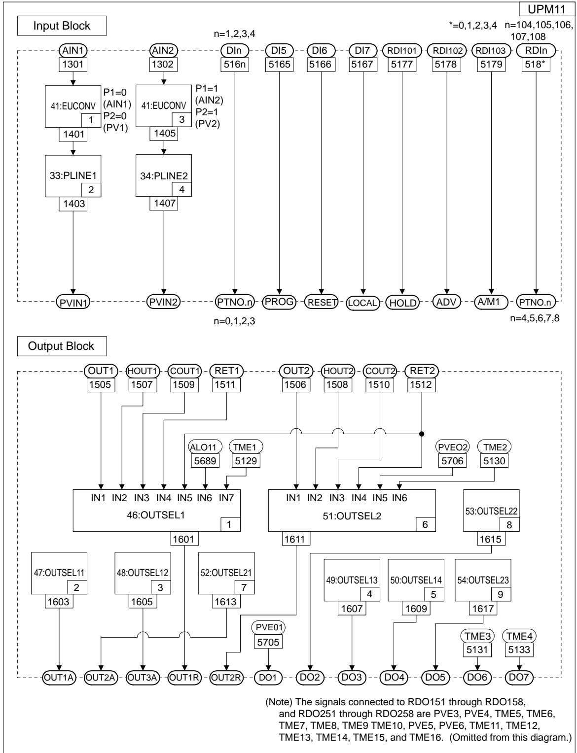
Figure 2.9 Input and Output Blocks for Dual-loop Control (UP Mode 11)
