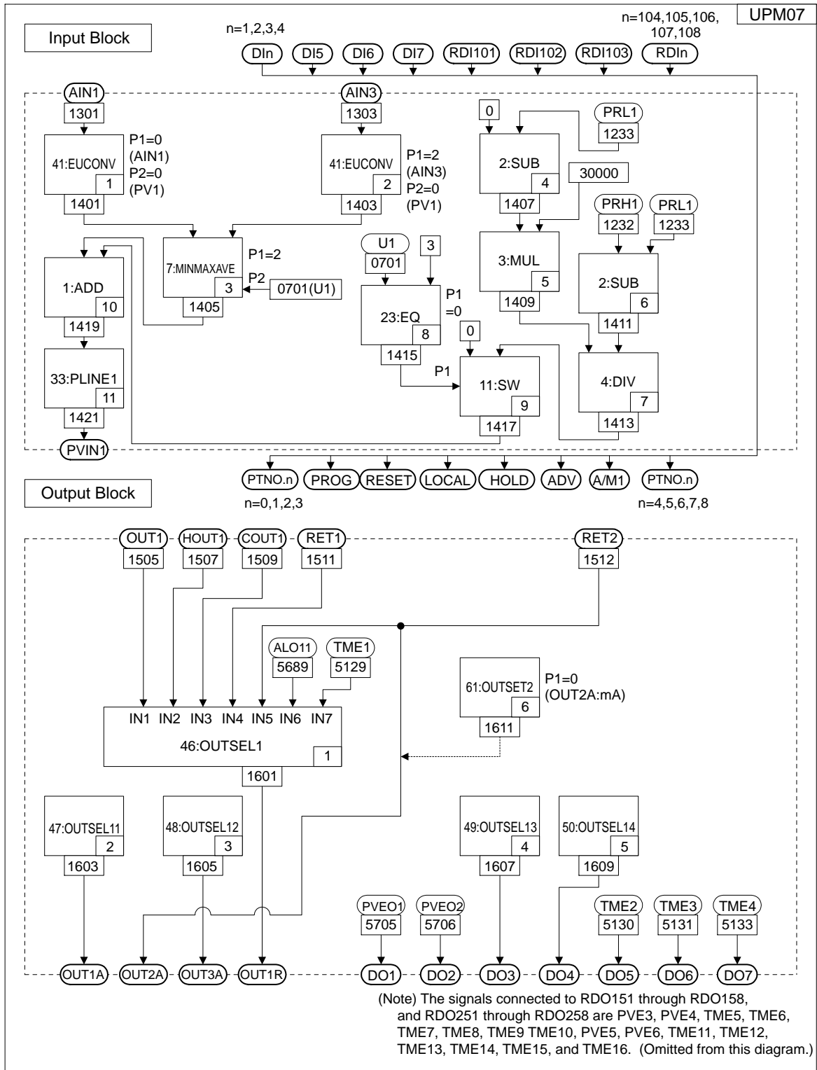
Figure 2.8 Input and Output Blocks for Loop Control with PV Auto-selector (UP Mode 7)
